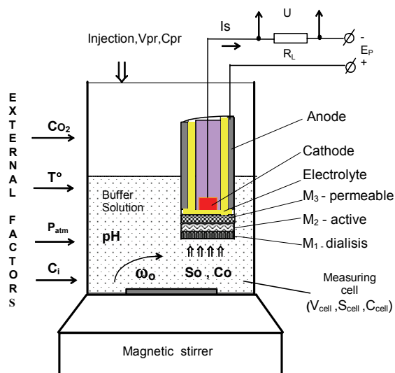
Fig. 1. Schematic representation of the dual-electrode experimental setup
