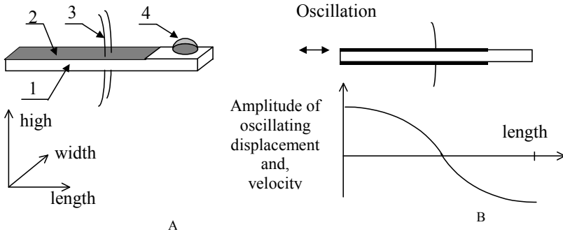
Fig. 5. Design and oscillation mode of a quartz resonator. A is a quartz resonator with a drop of studied liquid, 1 is a quartz plate, 2 is the metallization, 3 is the supporting conductors, and 4 is a drop of studied liquid. B is the distribution of the oscillatory velocity amplitude and longitudinal displacement.
