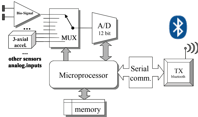
Fig. 4. System architecture
