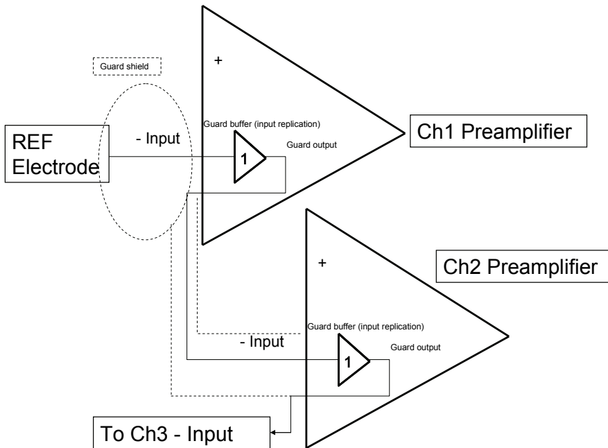
Fig. 8. Multi-channels wiring
